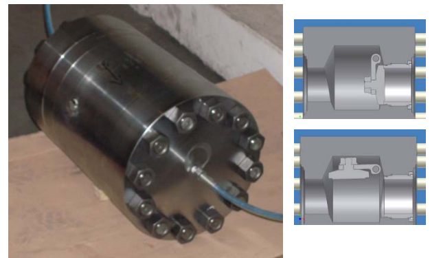
4" 15M CF Series Check Valve (Metal Seated) Gas Testing per API 6A PSL-3G
